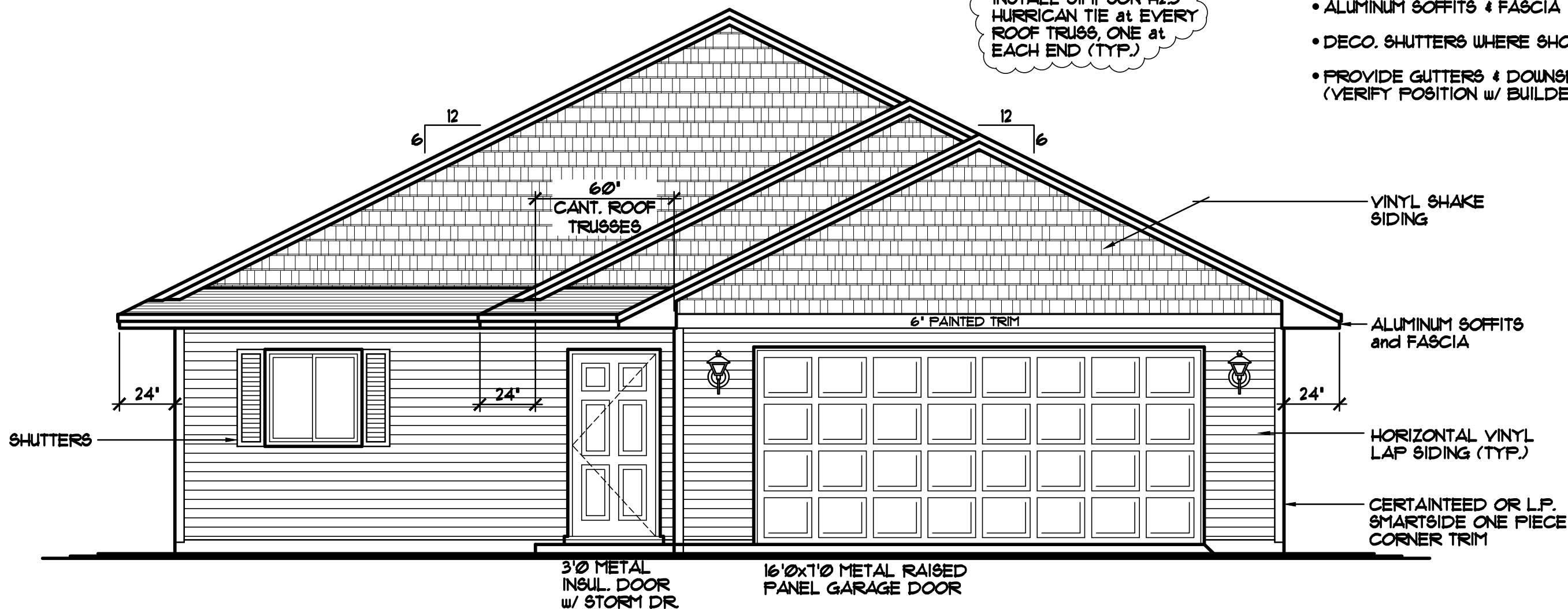
FRONT ELEVATION 1/4"=1'-0" 1400 SQFT. MAIN LEVEL
