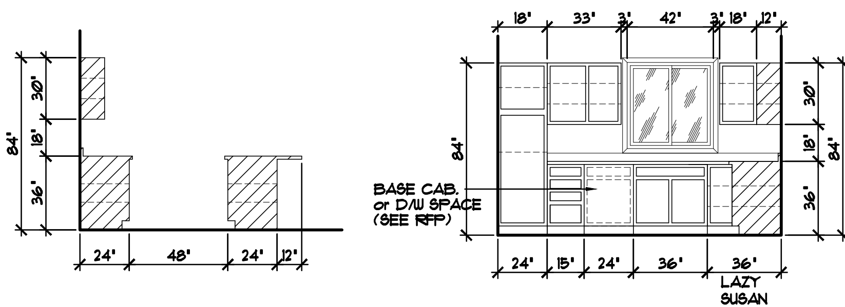
KITCH. CAB. ELEV. 1/4"=1'-0"
