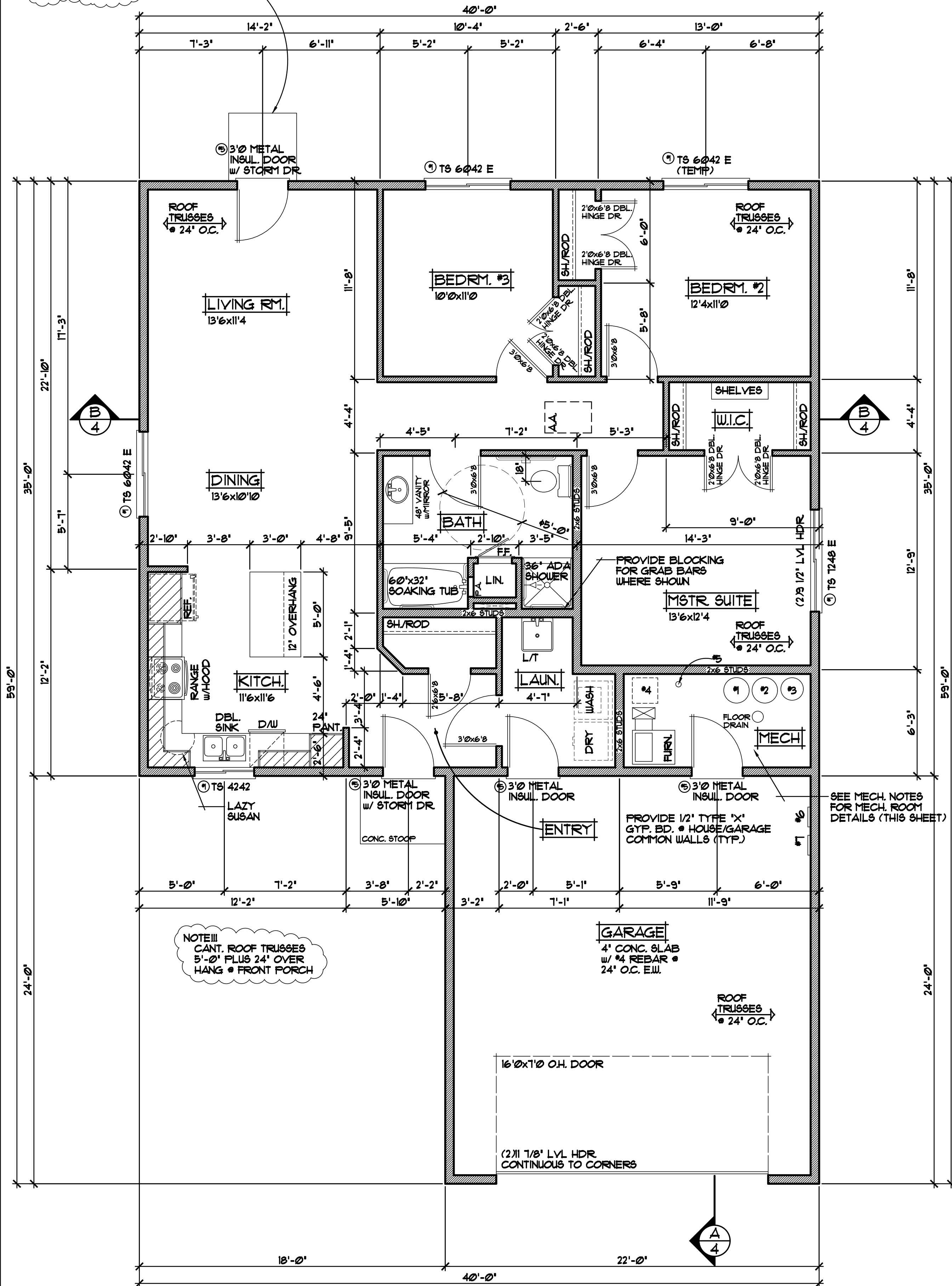
MAIN LEVEL FLOOR PLAN 1/4"=1'-0" 1400 SQ.FT.
