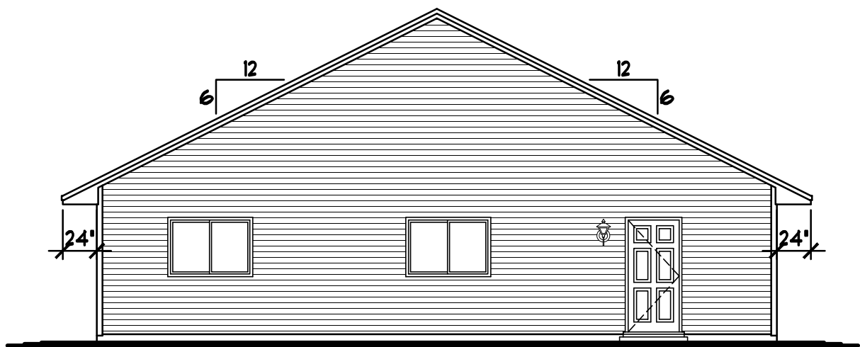
REAR ELEVATION 1/8"=1'-0"
