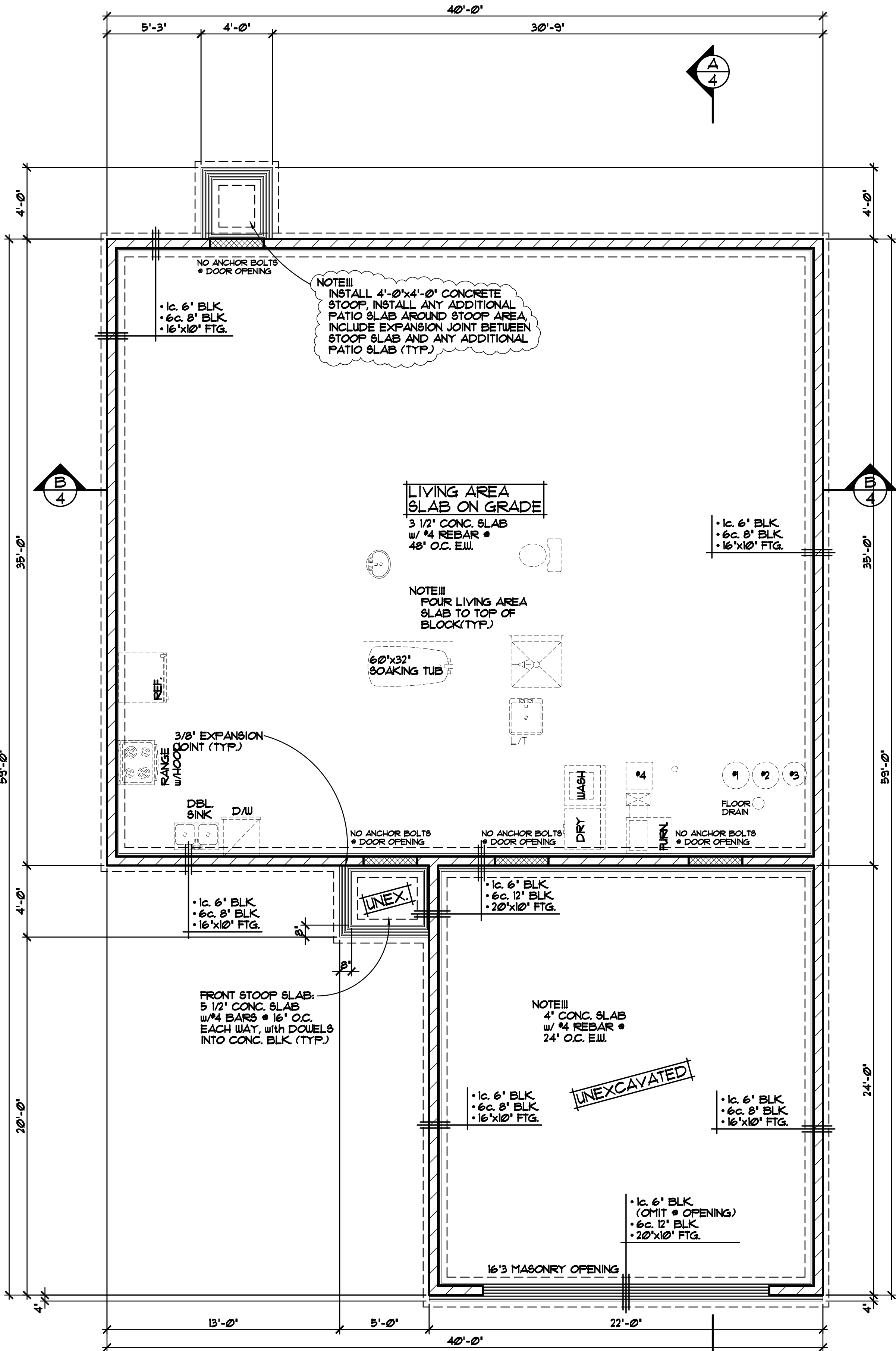
FOUNDATION PLAN 1/4"=1'-0"
