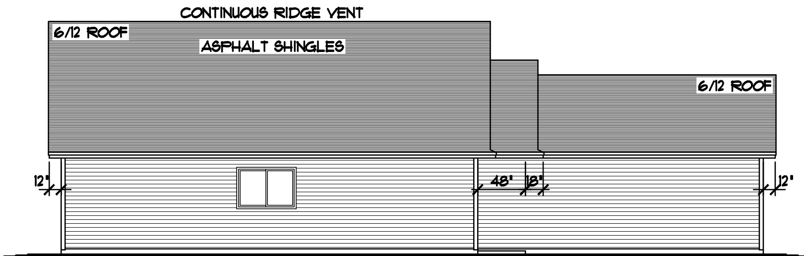
LEFT ELEVATION 1/8"=1'-0"
