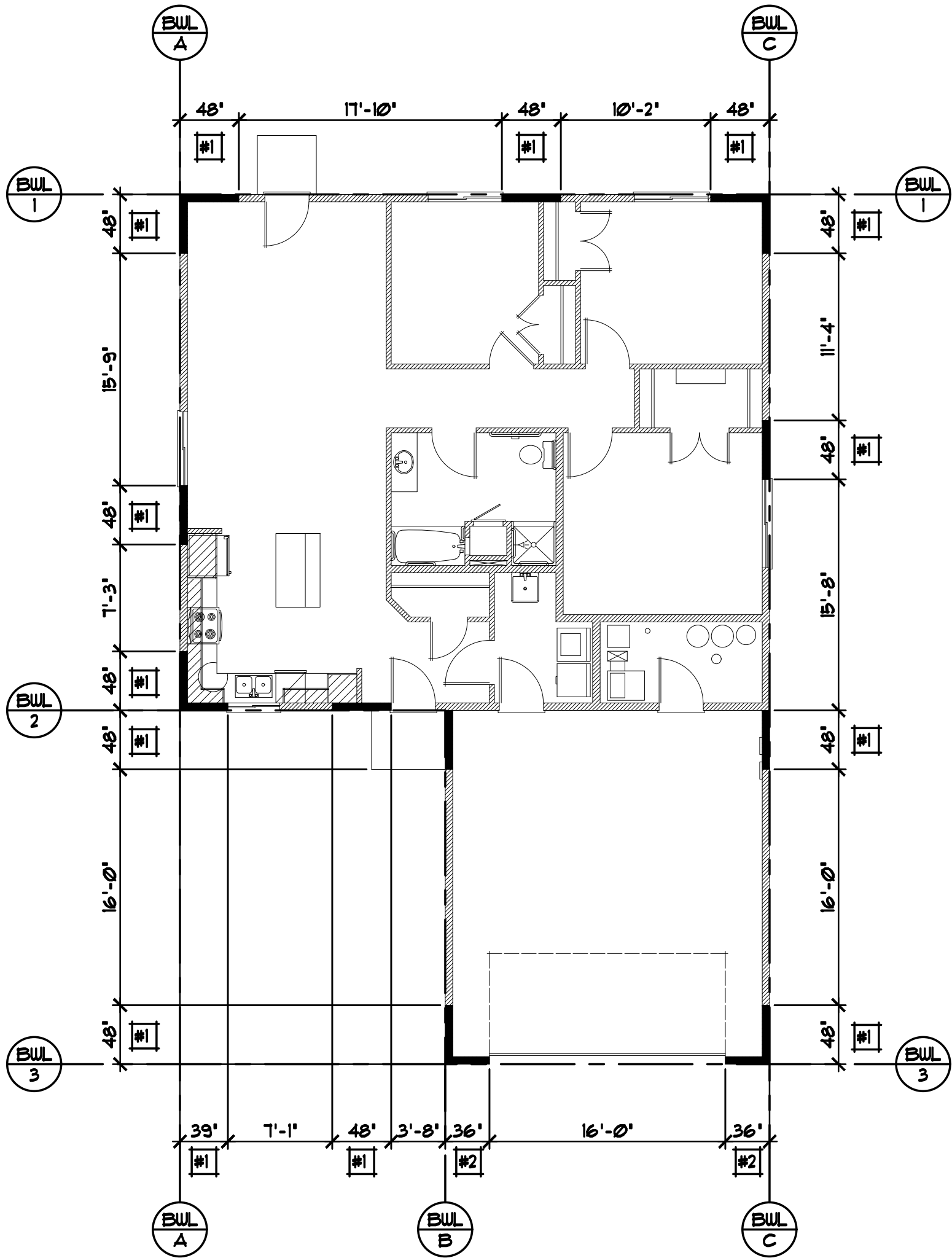
MAIN LEVEL WALL BRACING PLAN 1/8"=1'-0"
