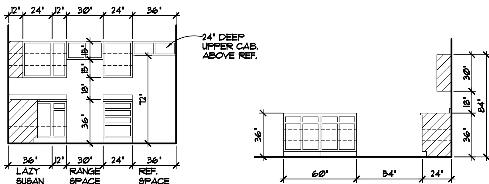
KITCH. CAB. ELEV. 1/4"=1'-0"
