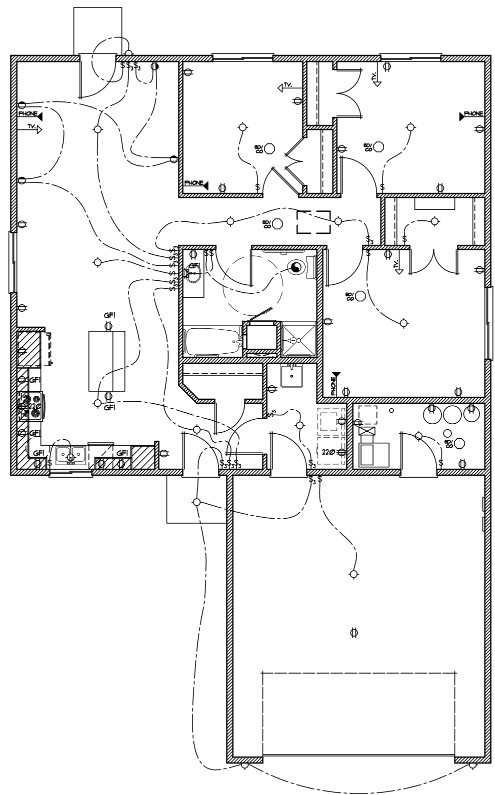
ELECTRICAL PLAN 1/8"=1'-0"
