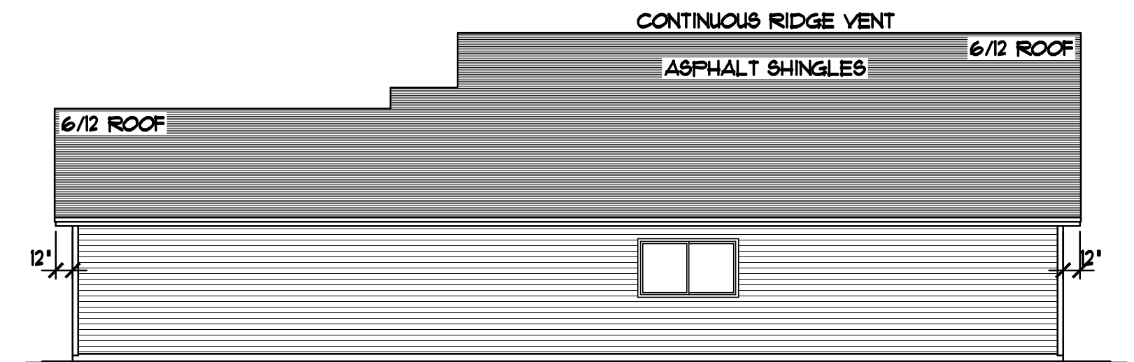
RIGHT ELEVATION 1/8"=1'-0"
