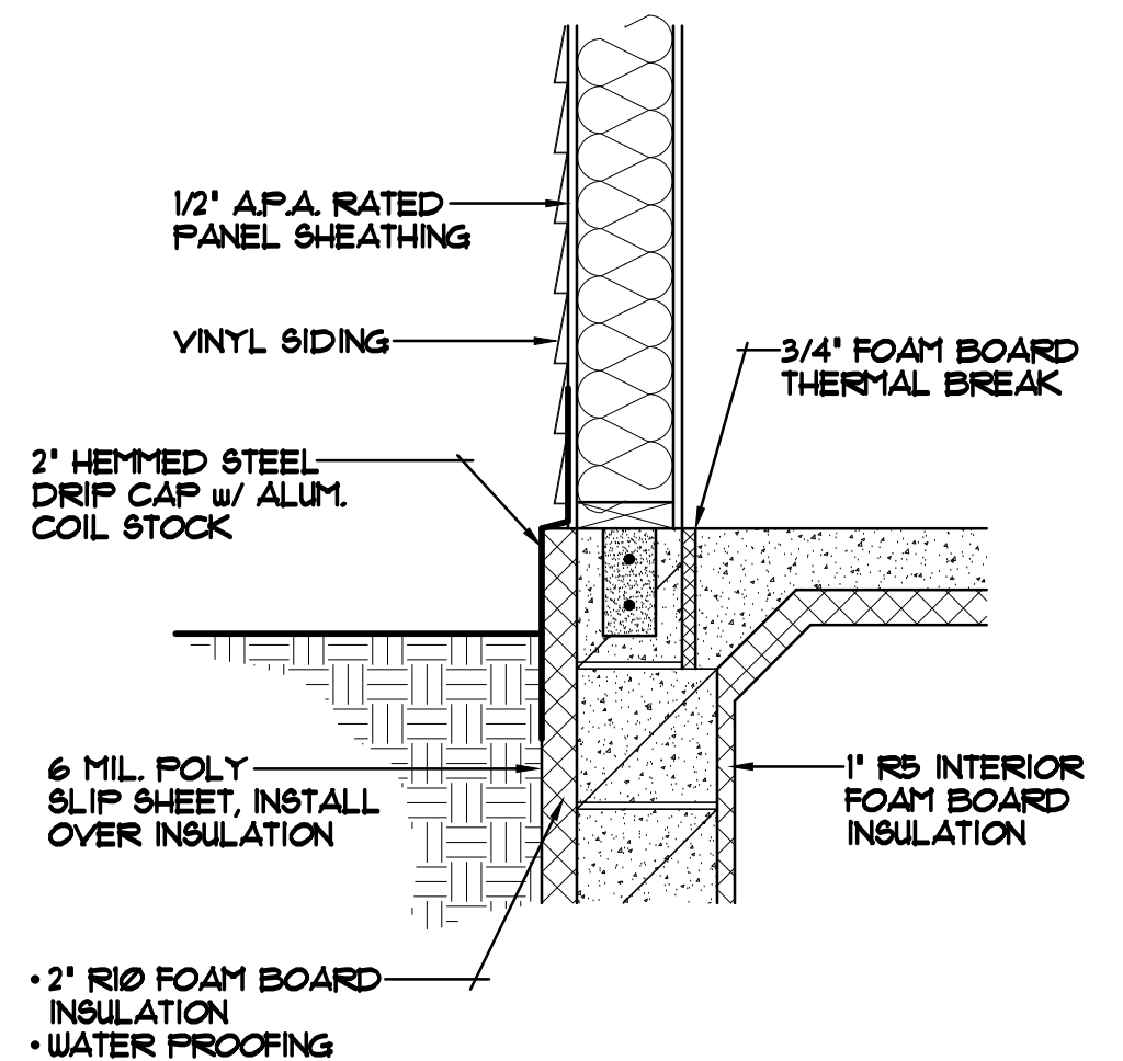
FOUNDATION FLASHING DETAIL
